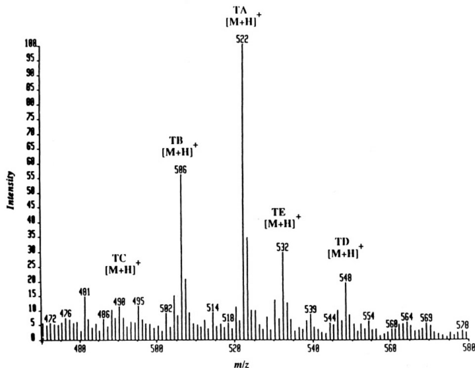
Figure 2. Positive ion FAB spectrum of AAL toxins isolated from culture filtrate using conditions described in the text. Protonated molecules are observed for the five toxins TA, TB, TC, TD, and TE.
