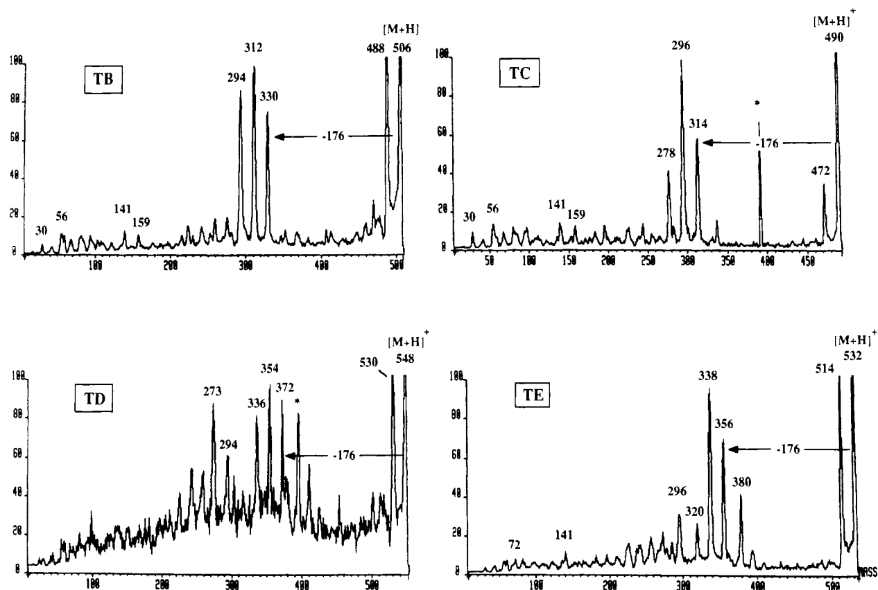
Figure 3. Daughter CAD/MIKE spectra for AAL toxins TB (B), TC (C), TD (D), TE (E). Spectra were obtained using conditions described in the text. Fragment ions attributed to the FAB matrix are labeled with an asterisk (*).
