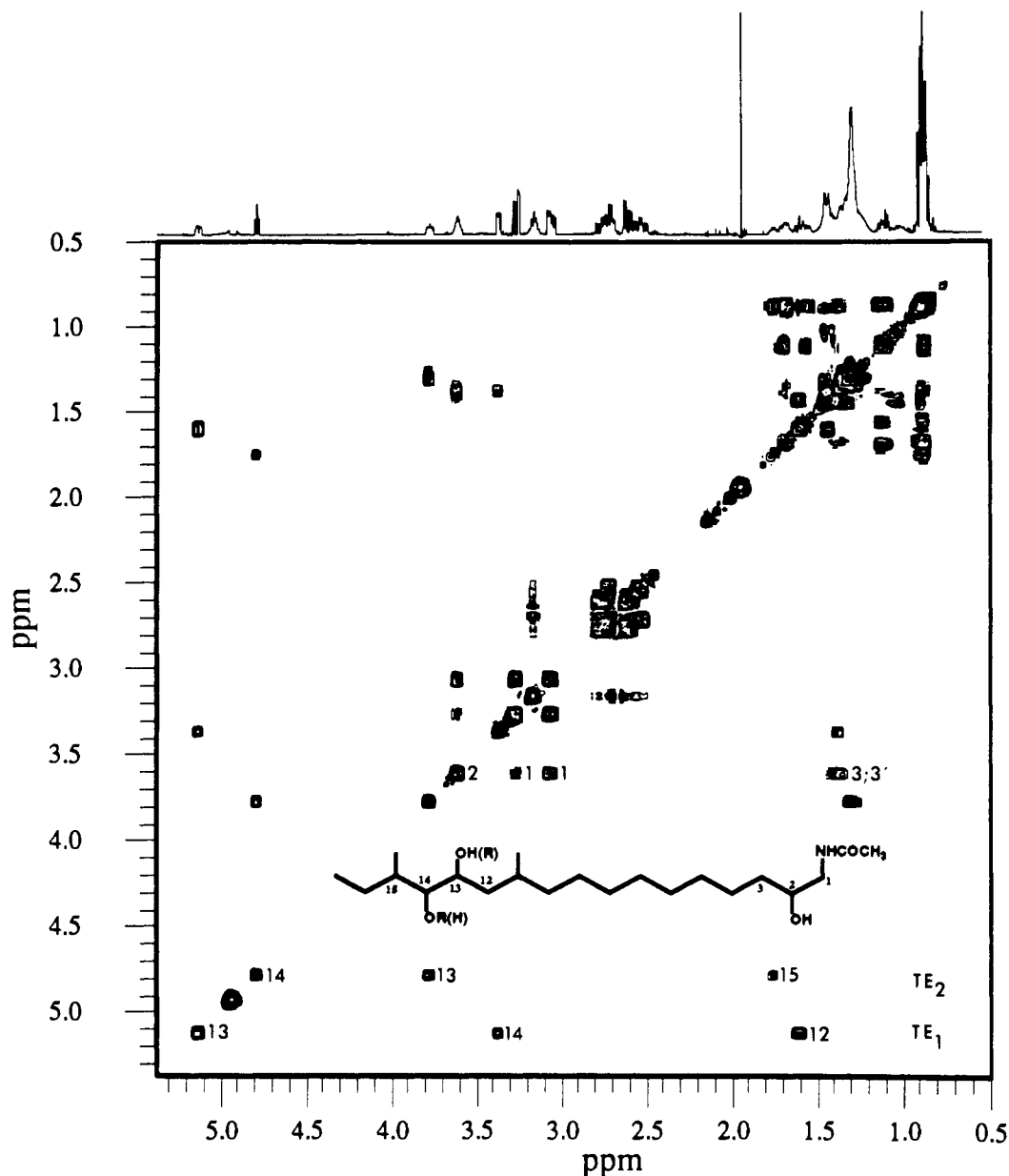
Figure 4. COSY spectra of TE showing the coupling patterns of the hydrogens at C 12 , C 13 , C 14 , and C 15 of isomers TE 1 and TE 2 and the coupling of the hydrogens at C 1 , C 2 , and C 3 in both isomers. The diagonal represents a contoured one-dimensional spectrum. The enumerated off-diagonal resonances represent the proton-proton coupling of the hydrogens at C 13 and C 14 of isomers TE 2 and TE 1 and the coupling of the hydrogens at C 2 in both isomers.
